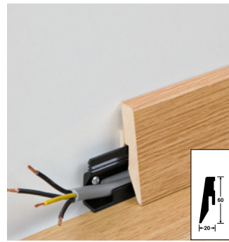
Skirting board profile 3 PK (60mm)
