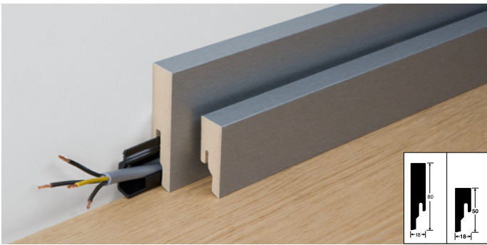
Skirting board profile 9 PK (80mm), profile 8 PK (50mm)
