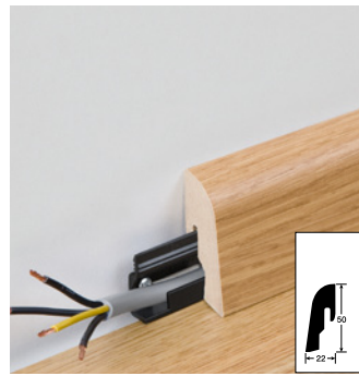
Skirting board profile 2 PK (50mm)
