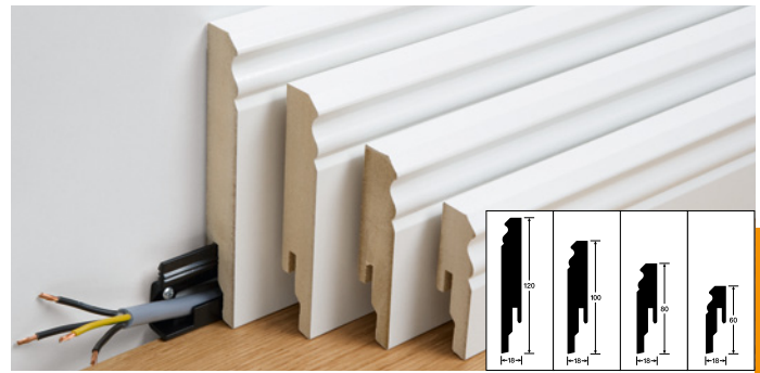
Skirting board profile 13 PK (120mm), 12 PK (100mm), 11 PK (80mm), 10 PK (60mm)
